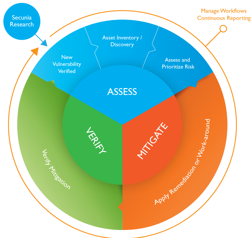
Figure 1: The Software Vulnerabilities Management Lifecycle
